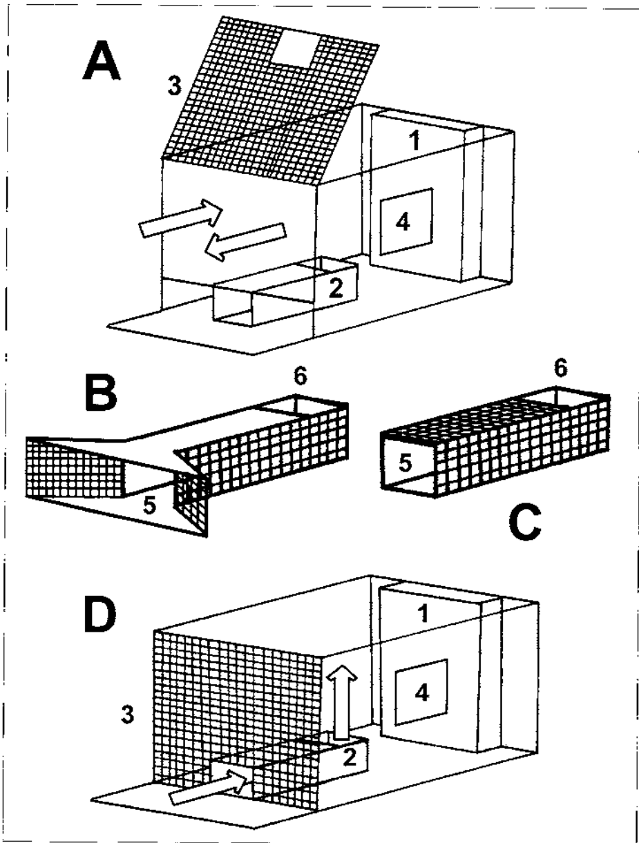
Figure 1. Funnel trap design. A) Lateral view in free access position. B) & C) Tunnel (5: access to funnel; 6: access into trap from funnel). D) Lateral view in activated position (1: feeder; 2: funnel; 3: door; 4 door for extracting birds).
